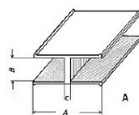
H-lood 12 x 4,5 - lengte 1.8 meter (LOH12x45M2)
