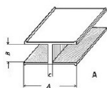
H-lood 10 x 4,5- kist 25 kg á 1.8 meter (LOH10x45KG25)
