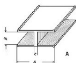
H-lood 8 x 5 - lengte 1.8 meter (LOH8x5M2)
