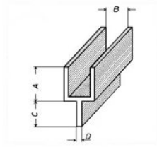
Y-lood 8 x 5 - lengte 1.8 meter (LOY8x5M2)
