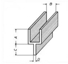
Y-lood 8 x 5- kist 25 kg á 1.8 meter (LOY8x5KG25)
