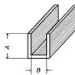
U-lood 8 x 4 - lengte 1.8 meter (LOU8x4M2)
