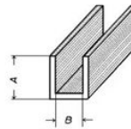
U-lood 6 x 4 lengte 2 meter (LOU6x4M2)
