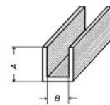
U-lood 8 x 5- kist 25 kg á 1.8 meter (LOU8x5KG25)
